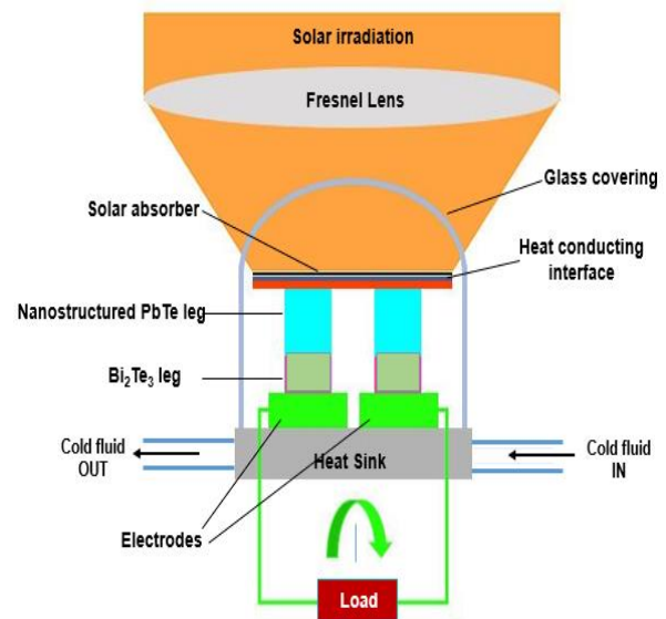
Fig. 1: Proposed System of Segmented PbTe/BiTe Legs STEG
