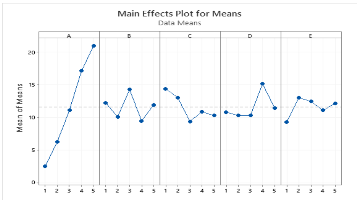
Fig. 2: Main Effect Plots for Power Output
