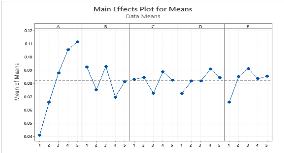
Fig. 3: Main Effect Plots for Conversion Efficiency
