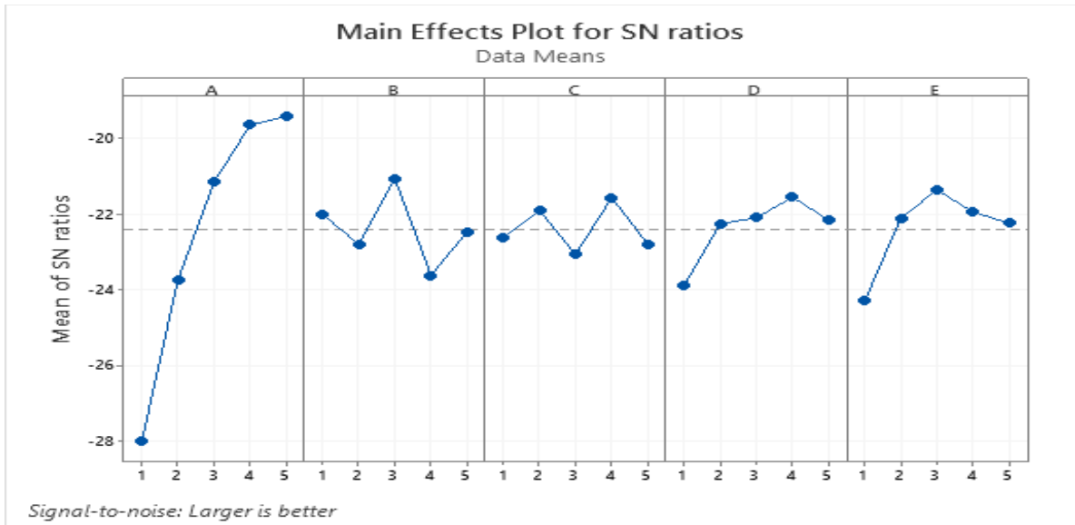
Fig. 5: Main Effect Plots of S/N Ratio for Efficiency
